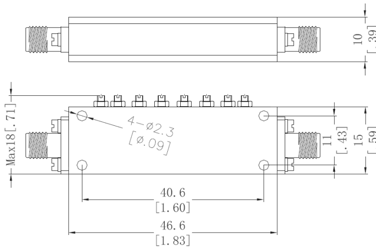
Physical Dimensions ( \pm 0.3\text{mm} )
